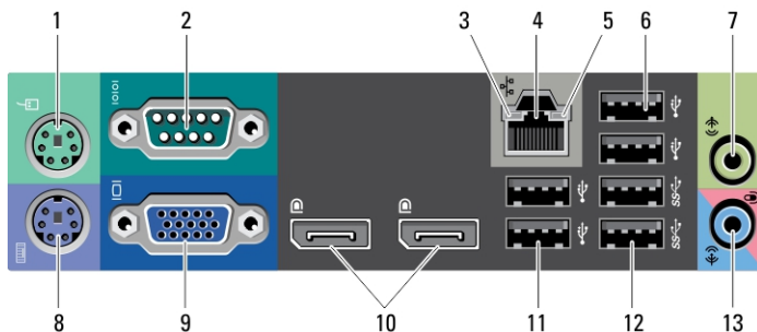
Figur 5. Small Form Factor set fra bagpanel
